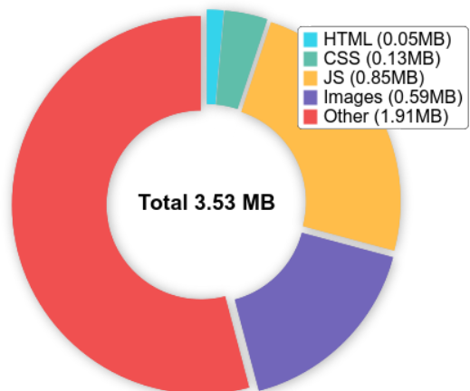
Page Size Breakdown
